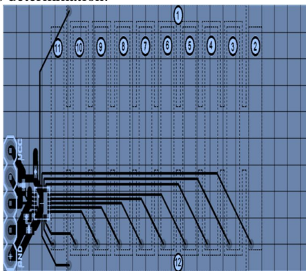
Figure. 2 PCB layout of capacitive sense board
