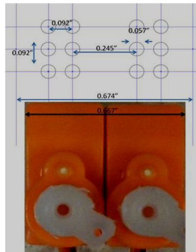
Figure. 1 Dimensions of servo
