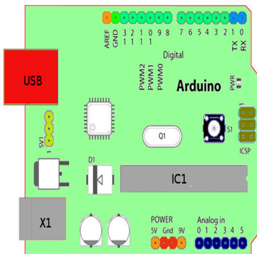
Figure. 4 Arduino board Specifications
