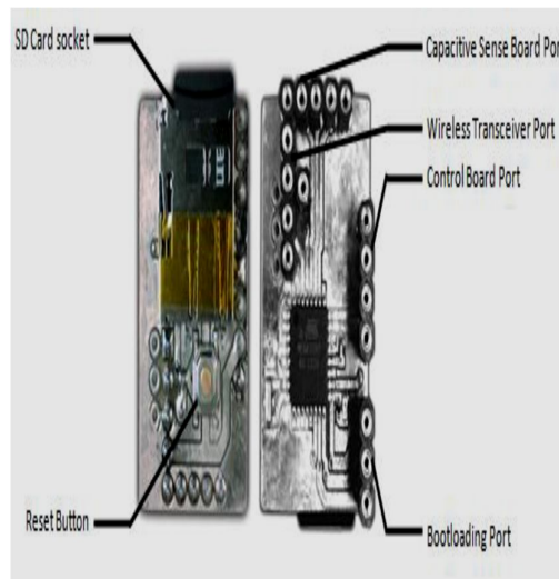
Figure. 3 sense board controller
