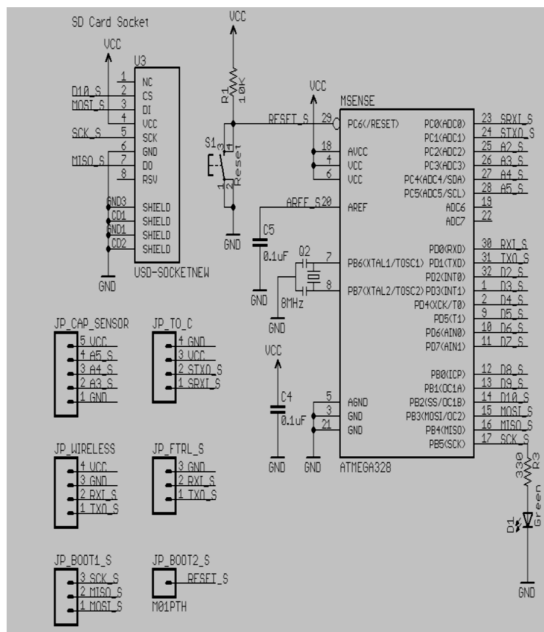
Figure. 5 Hardware Schematic
